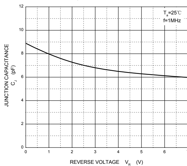
Capacitance Characteristics
